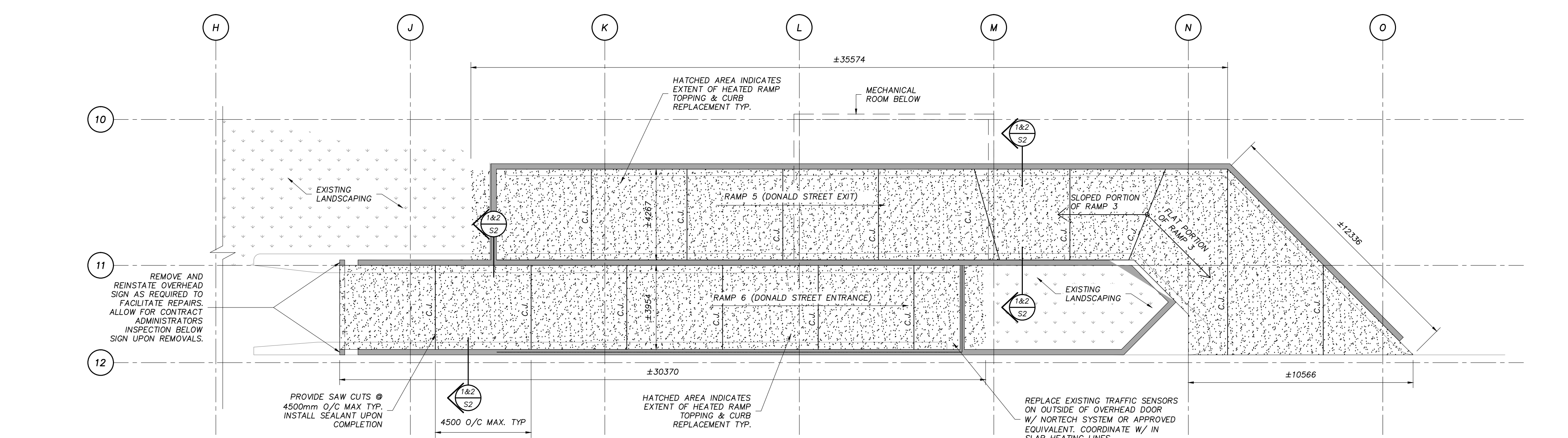
2 PARTIAL STREET LEVEL PLAN - DONALD STREET RAMPS SCALE: 1:125
